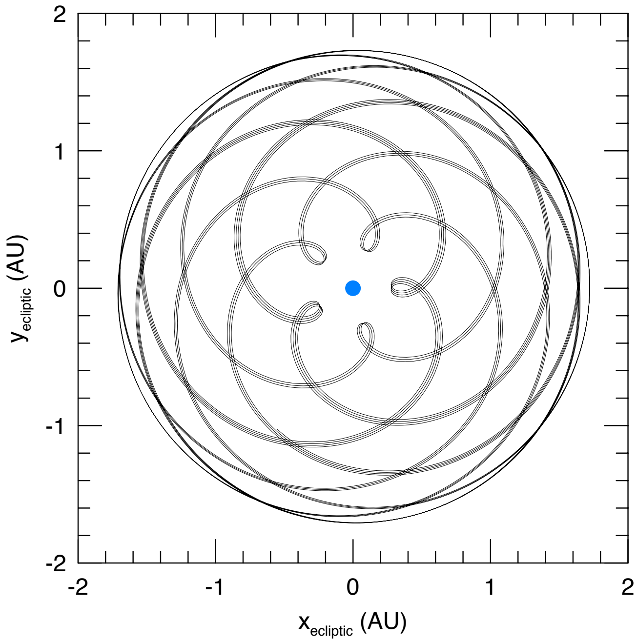
Orbit of Venus from a geocentric view over 100 years
