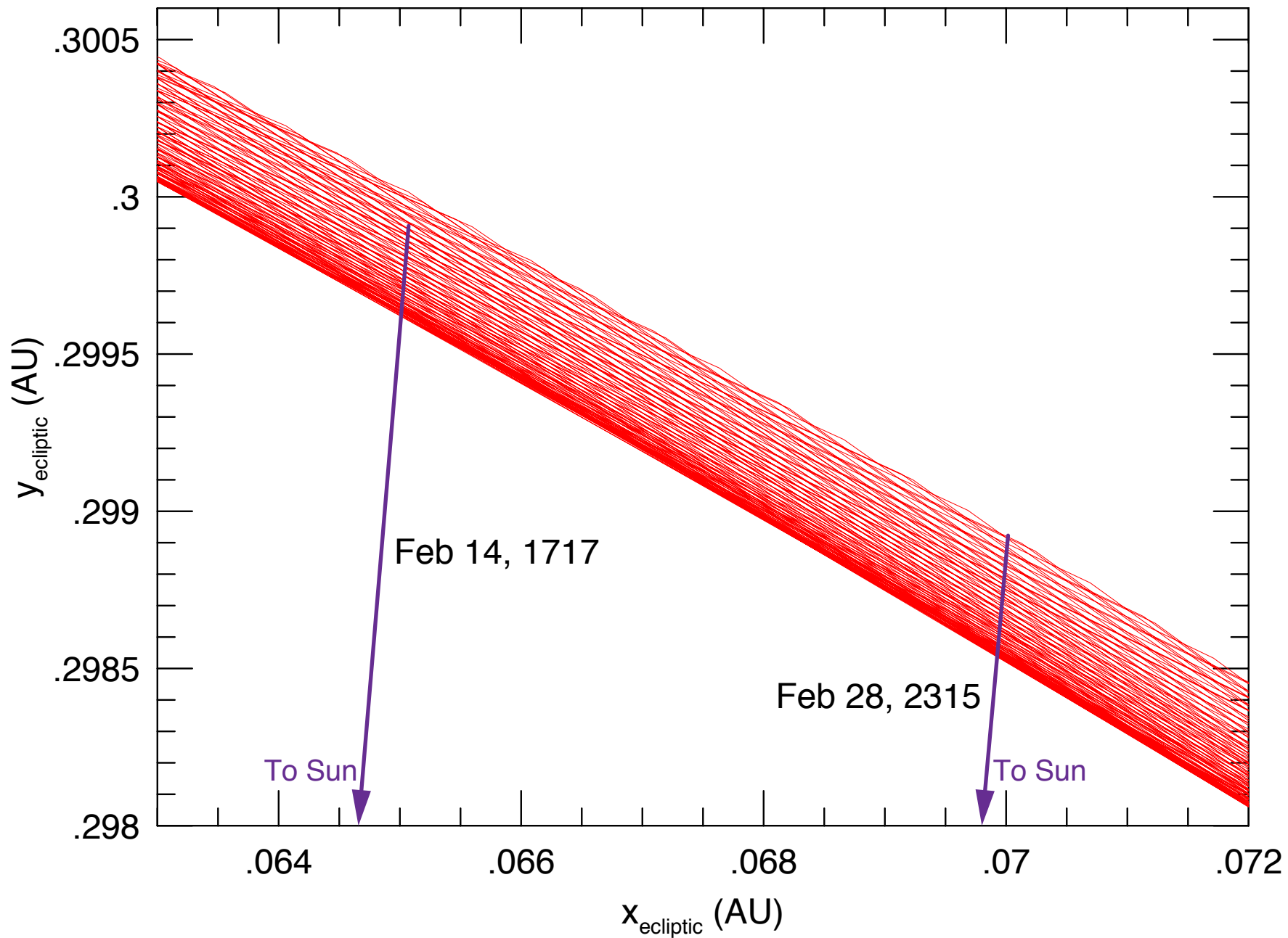
Advance of Perihelion, Mercury's orbits between 1717 and 2315
