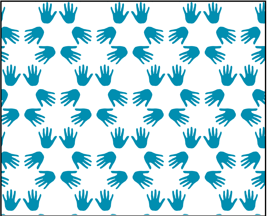
P3M1 Wallpaper
