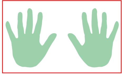
Lattice unit
