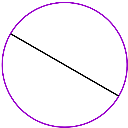
Geodesics of the Poincaré disc
