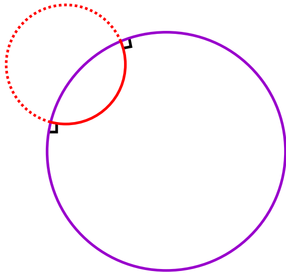
Geodesics of the Poincaré disc
