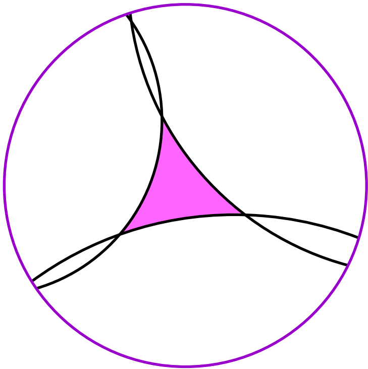
Triangles in the Poincaré disc
