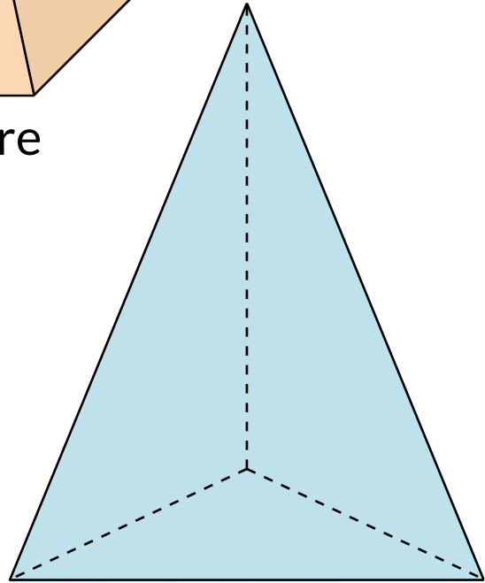
Right triangular pyramid
