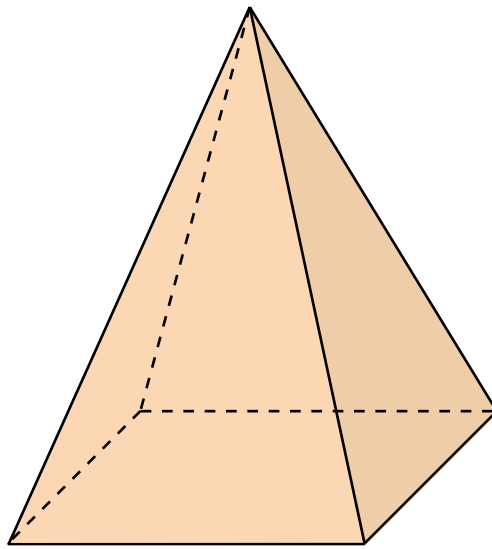
Right square pyramid
