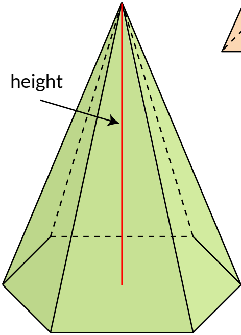
Right hexagonal pyramid
