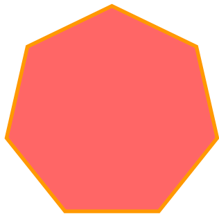
Regular Heptagon
