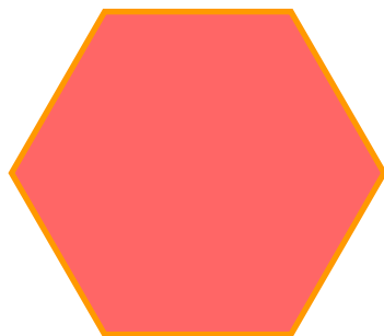
Regular Hexagon
