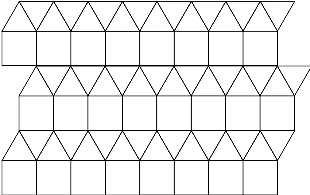
Tessellation
