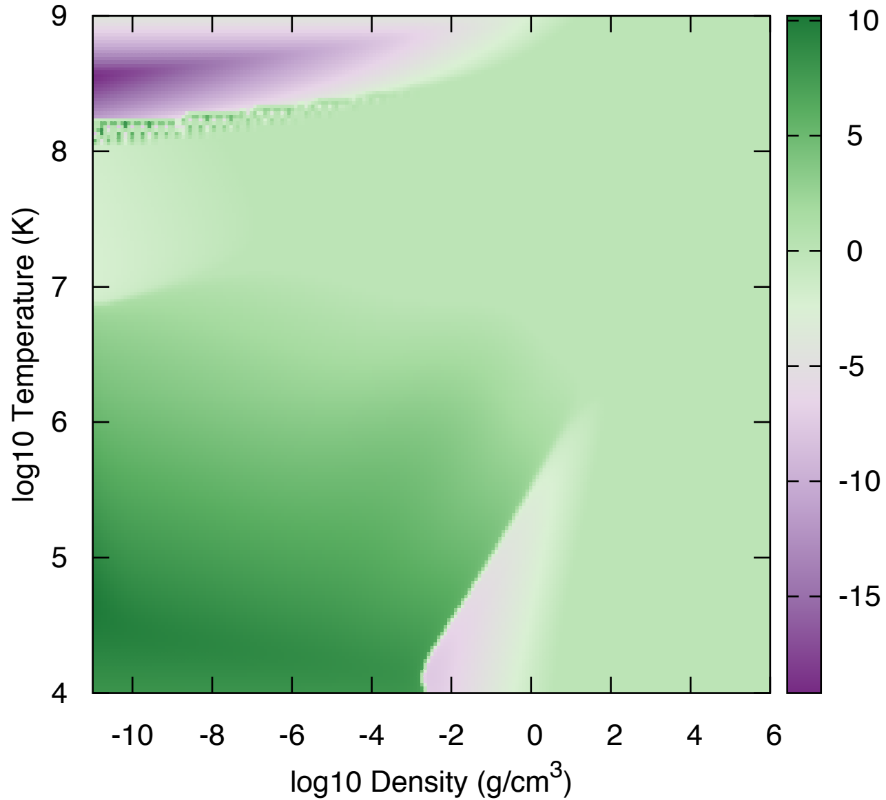
\log_{10} [ d(\text{opacity})/d(\rho) ] for Solar Mixture
