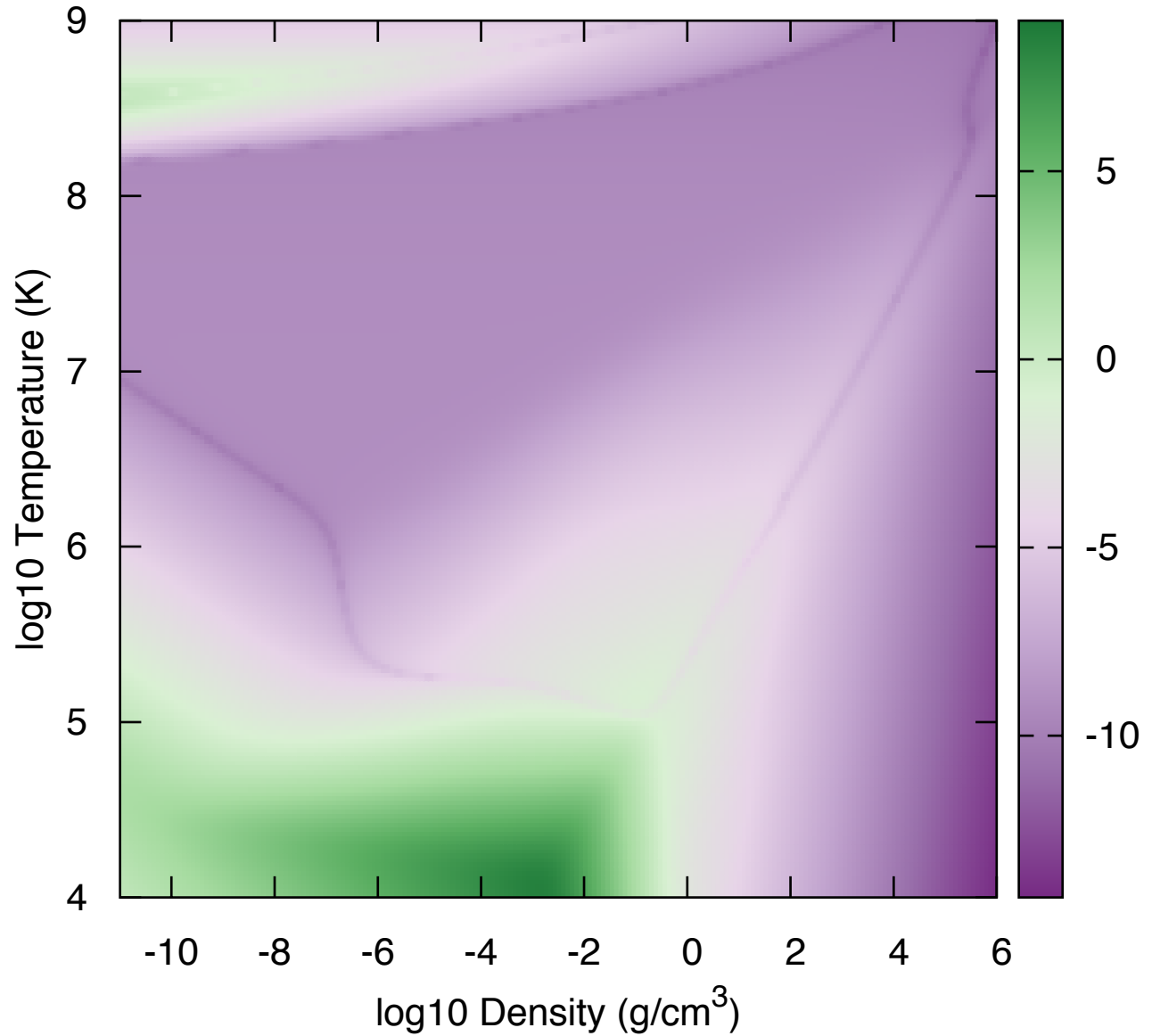
log10 [abs [d(opacity)/d(T)]] for Solar Mixture
