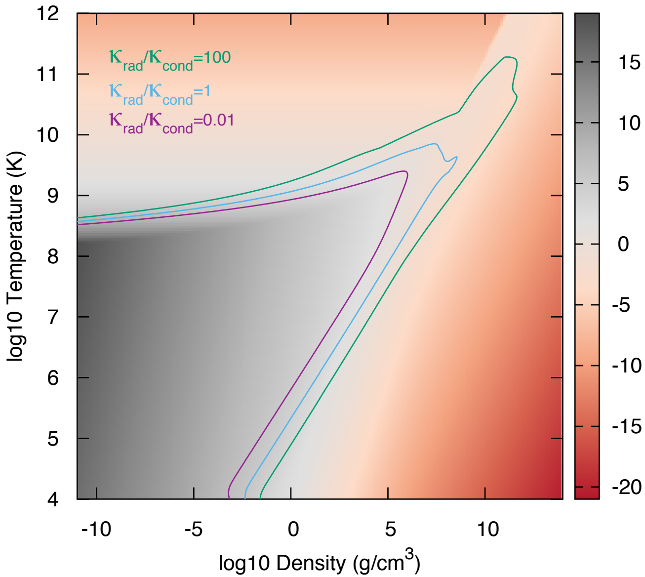
log10 (conductive opacity \text{cm}^2 \text{g}^{-1} ) for X(^{12}\text{C})=1
