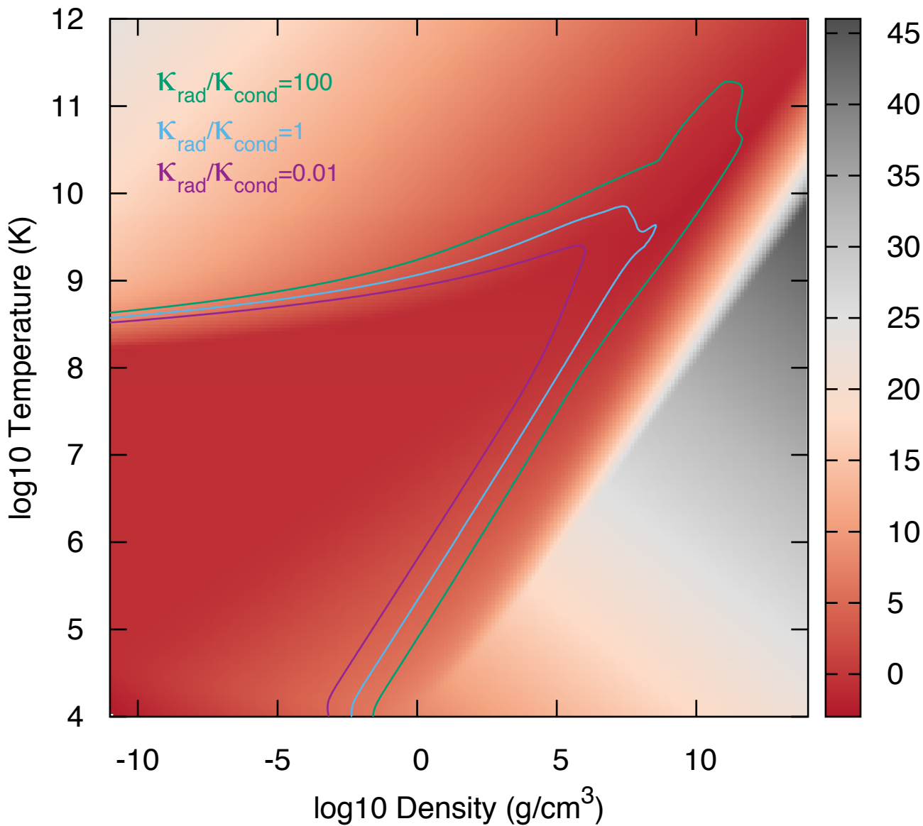
log10 (radiative opacity \text{cm}^2 \text{g}^{-1} ) for X(^{12}\text{C})=1
