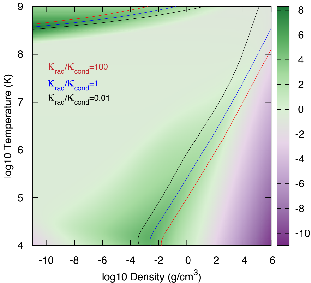
log10 (opacity \text{cm}^2 \text{g}^{-1} ) for Solar Mixture
