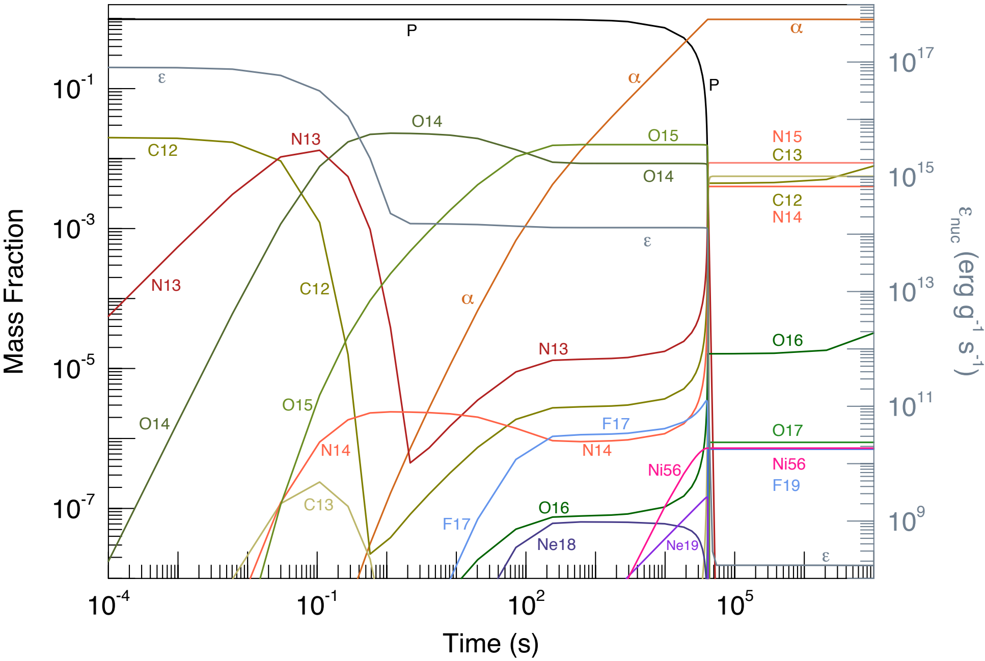
Beta Limited CNO cycles, hydrostatic burn, T=300 \times 10^6 K \rho=150 g cm ^{-3}
