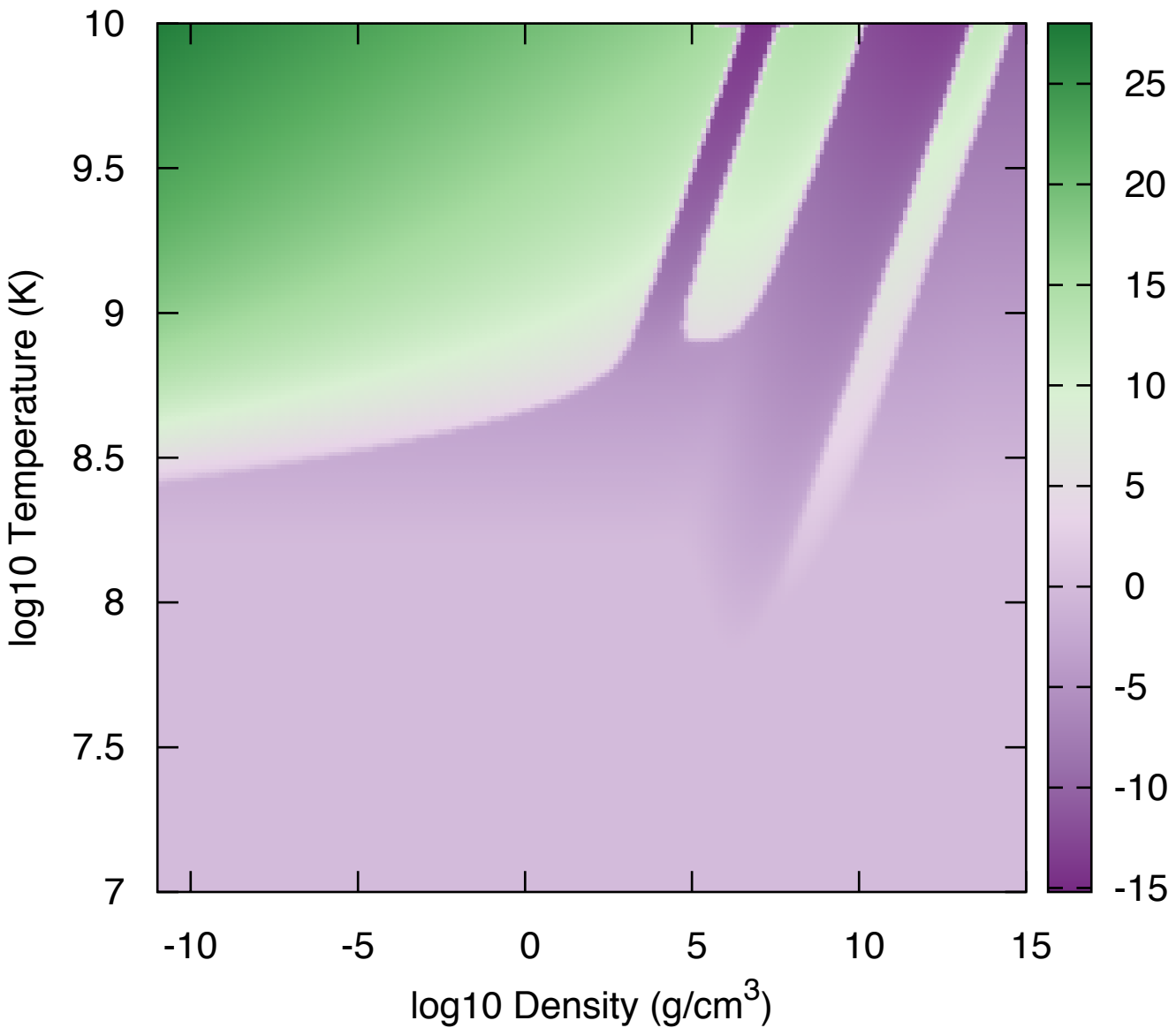
\log_{10} [(ds_{\text{neut}})/d(A_{\text{bar}})] for X(^{12}\text{C})=1
