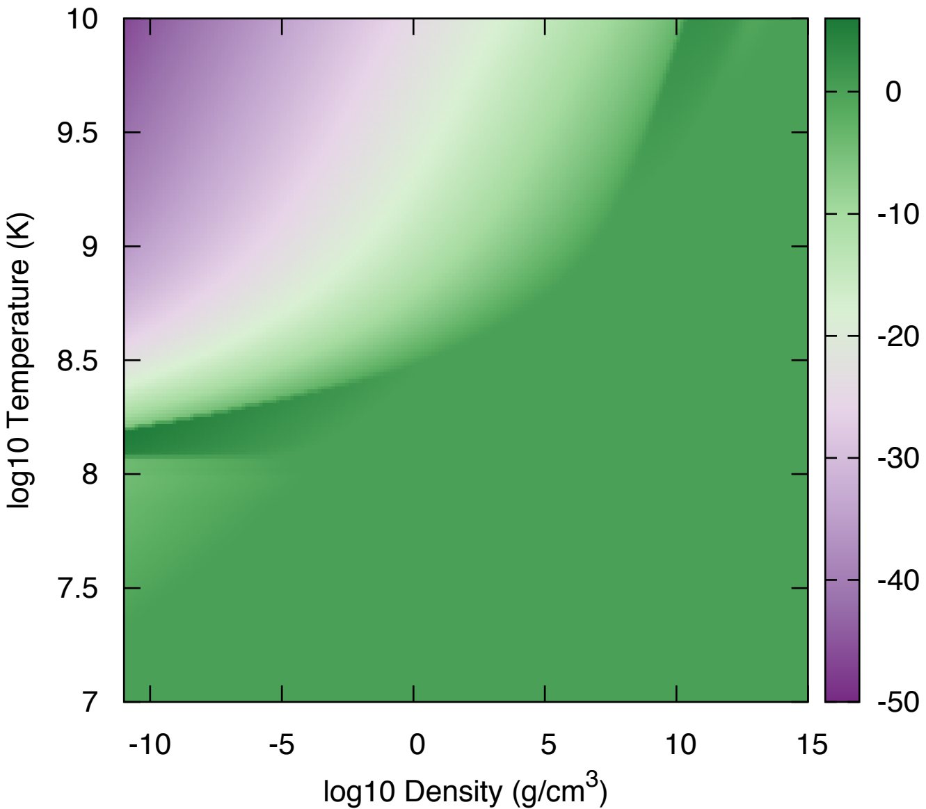
\log_{10} [(ds_{\text{neut}})/d(\rho)] for X(^{12}\text{C})=1
