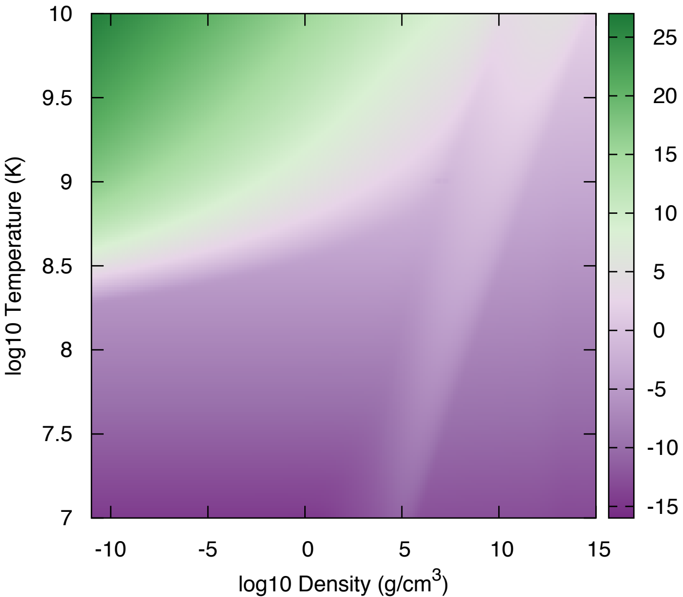
\log_{10} [(ds_{\text{neut}})/dT] for X(^{12}\text{C})=1
