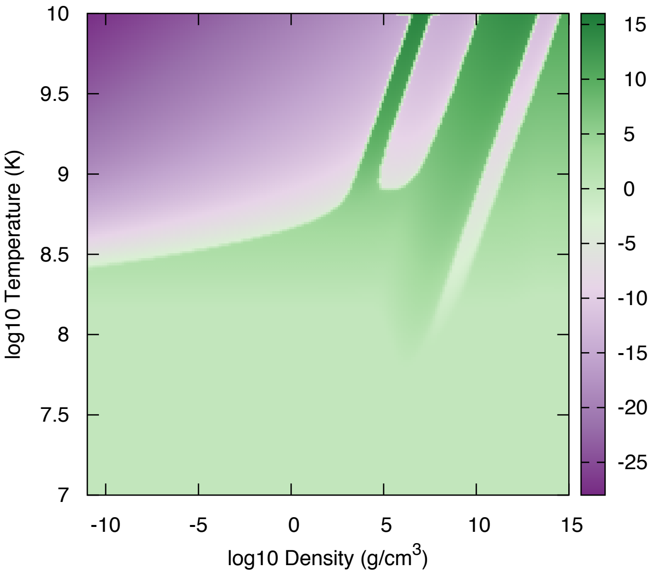
\log_{10} [(ds_{\text{neut}})/d(Z_{\text{bar}})] for X(^{12}\text{C})=1
